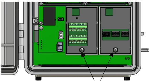
Tighten the screw on installed modules
